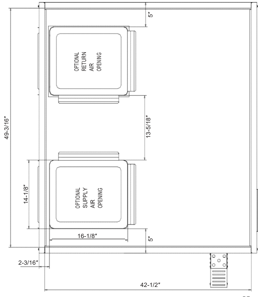
Bottom view
