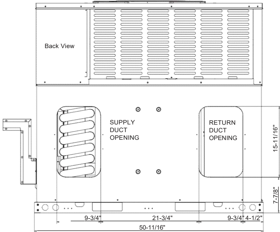
Back view
