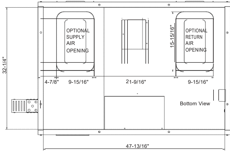
Bottom view
